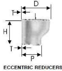
ECCENTRIC REDUCERS
